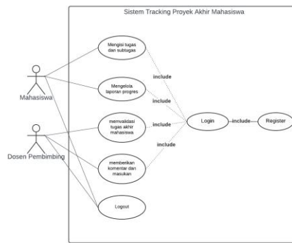
Gambar 7. Usecase Diagram
